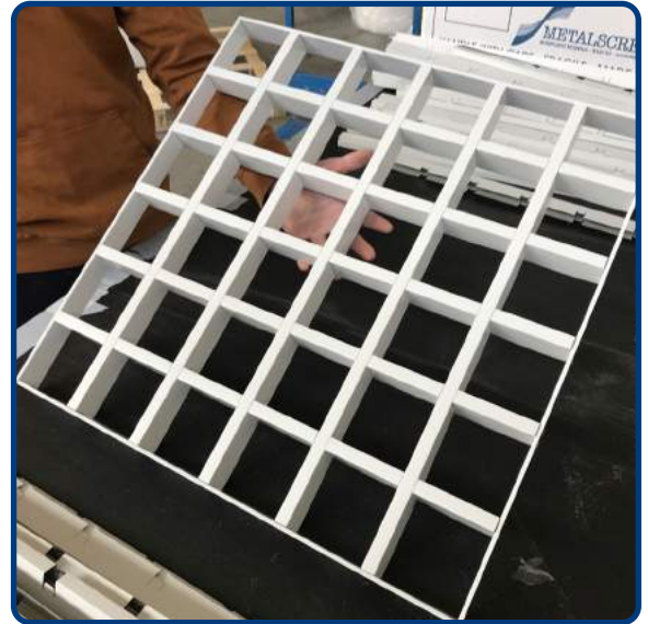
Capovolgere il pannello mm. 600x600 completo e assemblato Turn upside down the complete panel mm.600x600 assembled
